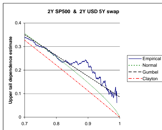
Figure 1.2: Estimated upper tail dependence coefficient for 2-year SP500 and USD swap futures.
