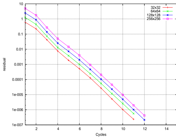
Figure 5. Multigrid convergence F(1,1)-cycle, \tau = 10^{-3} , pointwise-distributive.
