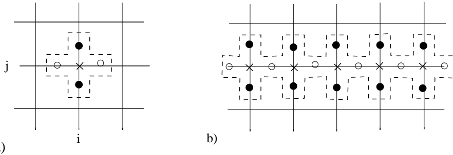
Figure 4. Five unknowns coupled smoothing: a): cellwise, b): x -linewise; \times : p_h , \circ u_h , \bullet : v_h .
