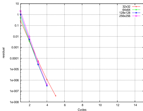
Figure 6. Multigrid convergence F(1,1)-cycle, \tau = 10^{-3} , linewise-distributive.
