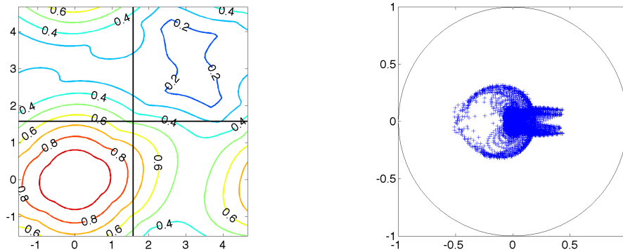
Figure 8. At left, the amplification factor for the diagonal pressure-wise Vanka smoother with under-relaxation on all variables with parameter \omega = 0.8 for the Q2-Q1 discretization of the Stokes equations on a mesh with h = \frac{1}{64} , as a function of the Fourier mode, \theta . At right, the spectrum of the two-grid error-propagation operator using this smoother with biquadratic interpolation for the velocities and bilinear interpolation for pressure.
