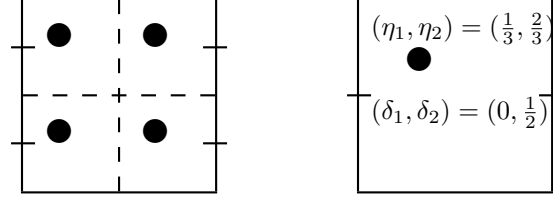
Figure 5. Nesting of fine-grid nodes relative to the coarse grid for non-nested grids, with (\delta_1, \delta_2) = (0, \frac{1}{2}) and (\eta_1, \eta_2) = (\frac{1}{3}, \frac{2}{3}) .
