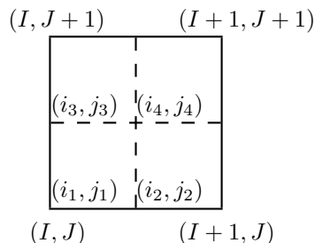
Figure 4. Nesting of fine-grid nodes relative to the coarse grid for nested (collocated) grids.
