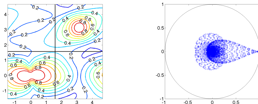
Figure 9. At left, the amplification factor for the element-wise (overlapping) Vanka smoother for the Q1-P0 discretization of the Stokes equations on a mesh with h = \frac{1}{64} , as a function of the Fourier mode, \theta . At right, the spectrum of the two-grid error-propagation operator using this smoother with bilinear interpolation for the velocities and piece-wise constant interpolation for pressure.
