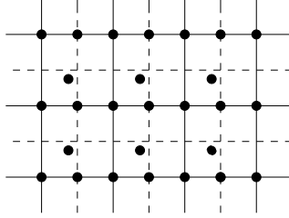
Figure 2. Partitioning of degrees of freedom into overlapping subsets based on cells
