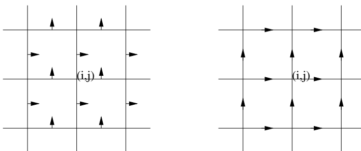
Figure 1. Placement of unknowns with Raviart-Thomas FE for grad-div operator (left), and Nédélec edge elements for curl-curl (right).
