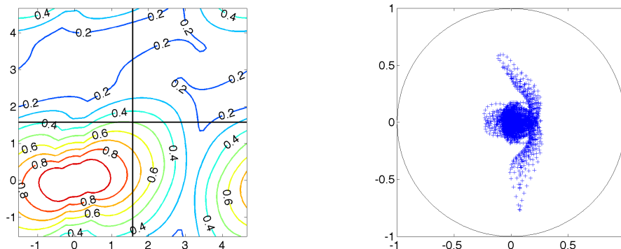
Figure 6. At left, the amplification factor for the full pressure-wise Vanka smoother with no under-relaxation for the Q2-Q1 discretization of the Stokes equations on a mesh with h = \frac{1}{64} , as a function of the Fourier mode, \theta . At right, the spectrum of the two-grid error-propagation operator using this smoother with biquadratic interpolation for the velocities and bilinear interpolation for the pressure.
