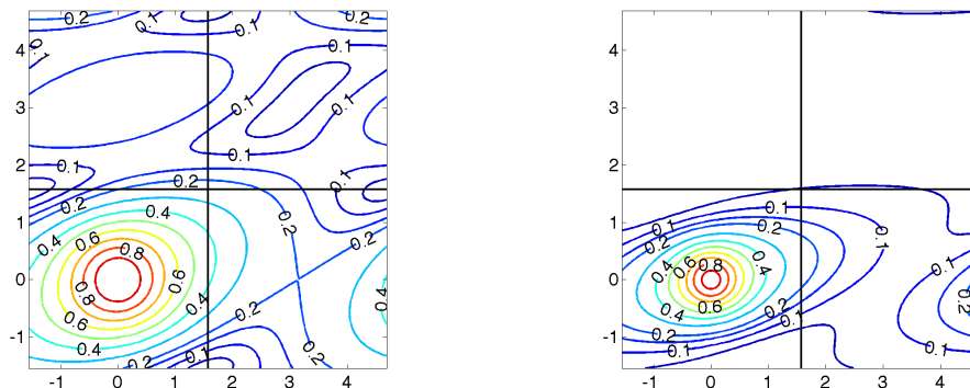
Figure 3. Amplification factors for pointwise Gauss-Seidel relaxation (at left) and element-wise overlapping multiplicative Schwarz (at right) for a Q1 discretization of the Poisson equation on a mesh with h = \frac{1}{128} , as a function of the Fourier mode, \theta .
