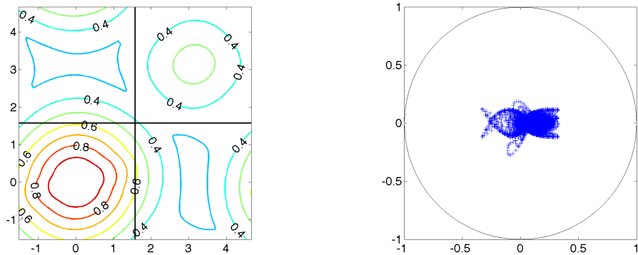
Figure 7. At left, the amplification factor for the full pressure-wise Vanka smoother with under-relaxation with parameter \omega = 0.5 used for the velocities only with the Q2-Q1 discretization of the Stokes equations on a mesh with h = \frac{1}{64} , as a function of the Fourier mode, \theta . At right, the spectrum of the two-grid error-propagation operator using this smoother with biquadratic interpolation for the velocities and bilinear interpolation for pressure.
